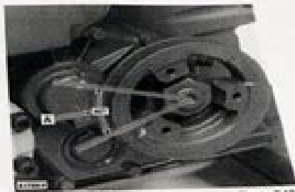
Crankshaft Rotated A 40° Figure 2-13
