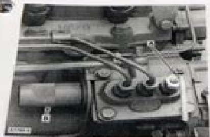
Spill Tube and Shut-Off Solenoid A Spill tube Figure 2-12
